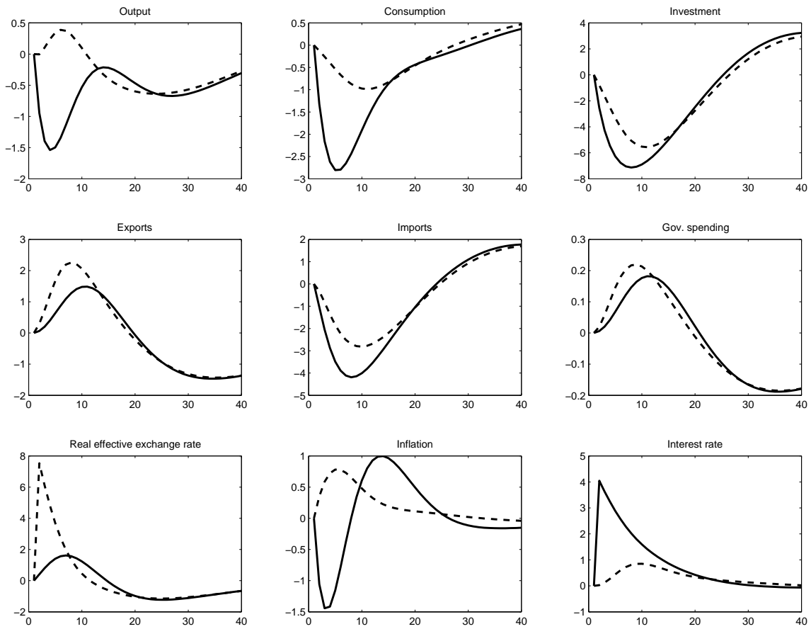
Figure 4: Impulse responses to a risk premium shock
