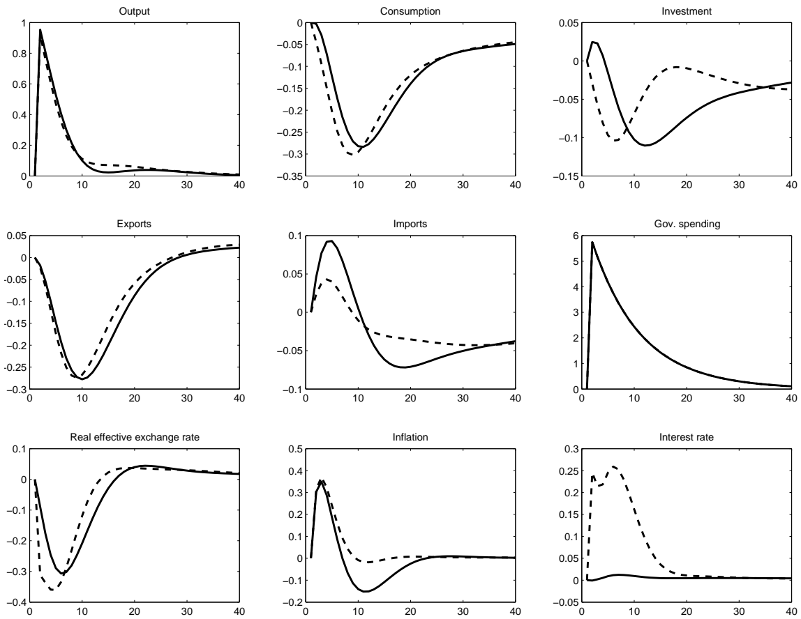
Figure 5: Impulse responses to a government expenditure shock
