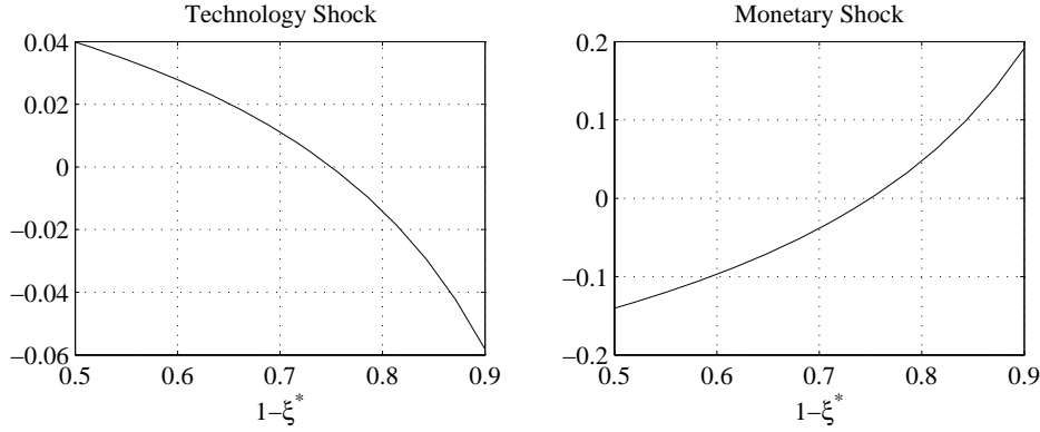
Figure 7: Impact Inflation Differential: \pi_c - \pi_c^*
