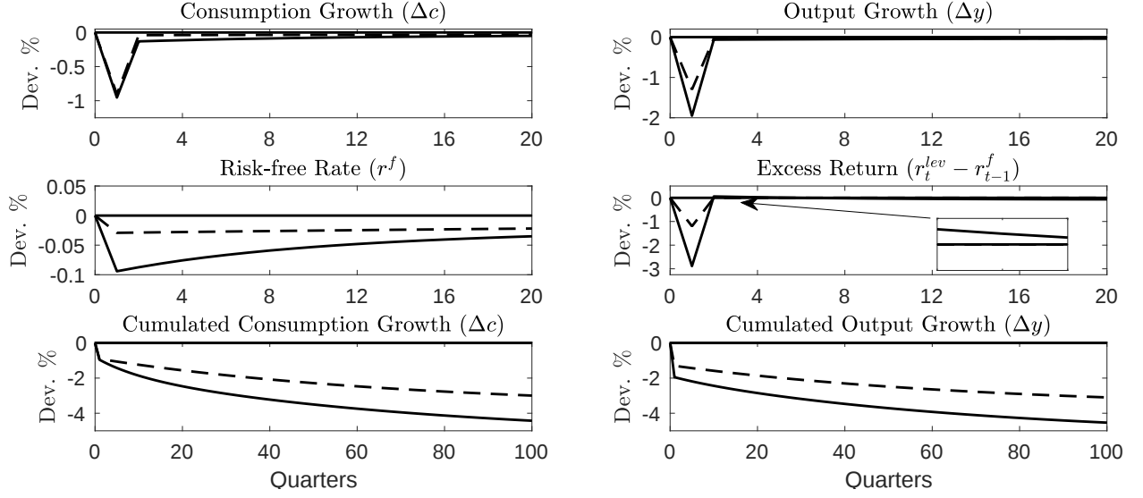
Figure 7: IRF Nested Models - II
